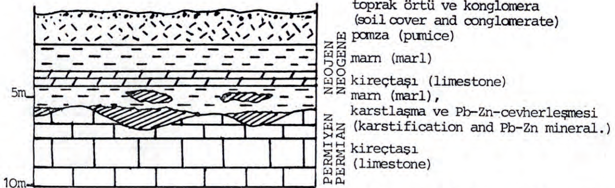
Figure 5 : Vertical sketch profile of Ağcaşar mine.
